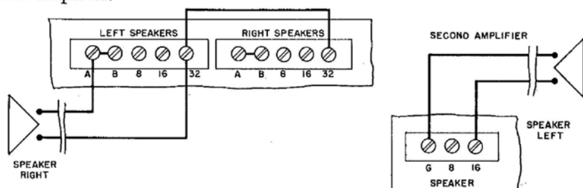
SPEAKER HOOK UP FOR STEREO CONVERSION
